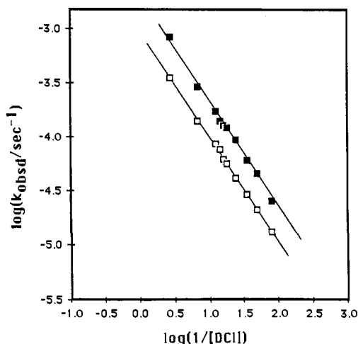
Figure 1. Double logarithmic plot of the rate constants for the reduction of N -(2,2,2-trifluoroethyl)- S,S -dimethylsulfilimine as a function of added acid concentration in H_2O ( \square ) and in D_2O ( \blacksquare ). Aqueous solution, 25 °C, [I^-] = 0.1 M, ionic strength 1.0 with KCl.
